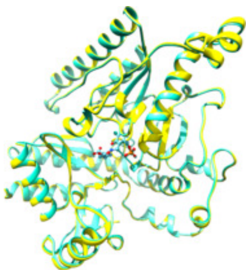
Figure 2. Ribbon diagram of the superimposed native GABA-AT (yellow) and GABA-AT (cyan) bound to CPP-115.
