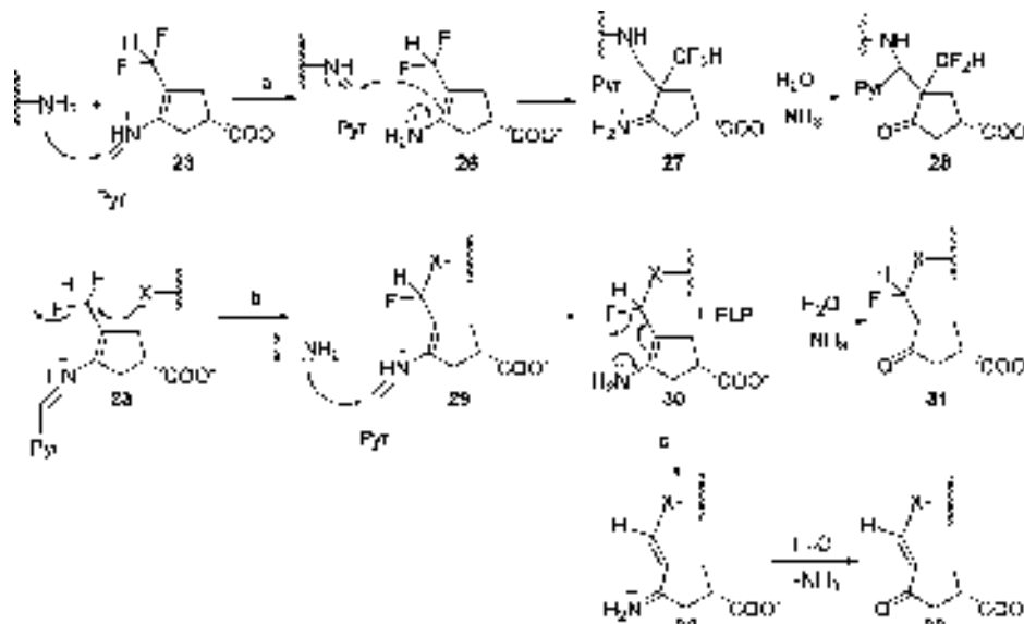
Scheme 7. Fourth Potential Mechanism of Inactivation of GABA-AT by CPP-115
