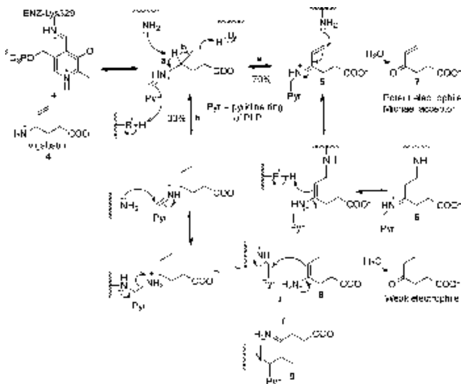
Scheme 3. Inactivation Mechanism of GABA-AT by Vigabatrins
