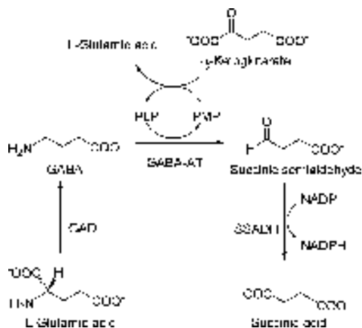
Scheme 1. GABA Metabolism 10
